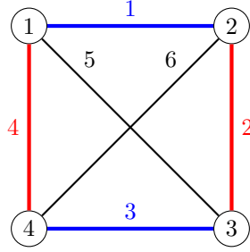
Figure 3: Example of a TSP solution. The blue and red perfect matchings together form a Hamiltonian cycle. The blue perfect matching has a weight of 1 + 3 = 4 , whereas the red perfect matching has a weight of 2 + 4 = 6 . The objective of the solution equals 4 + 6 = 10
